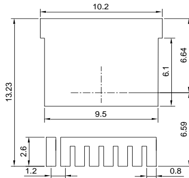
SUGGESTED SOLDER PAD LAYOUT TOP VIEW
