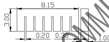
SUGGESTED SOLDER PAD LAYOUT
